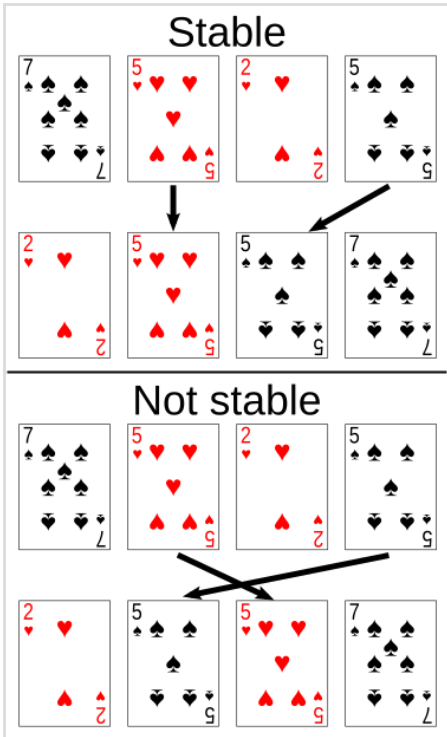
An example of stable sort on playing cards. When the cards are sorted by rank with a stable sort, the two 5s must remain in the same order in the sorted output that they were originally in. When they are sorted with a non-stable sort, the 5s may end up in the opposite order in the sorted output.
